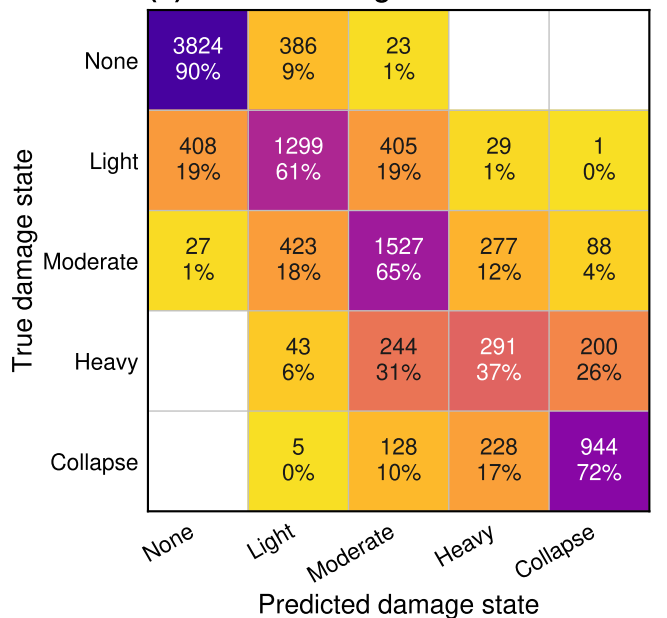
(b) EMS-98 damage-state classification
