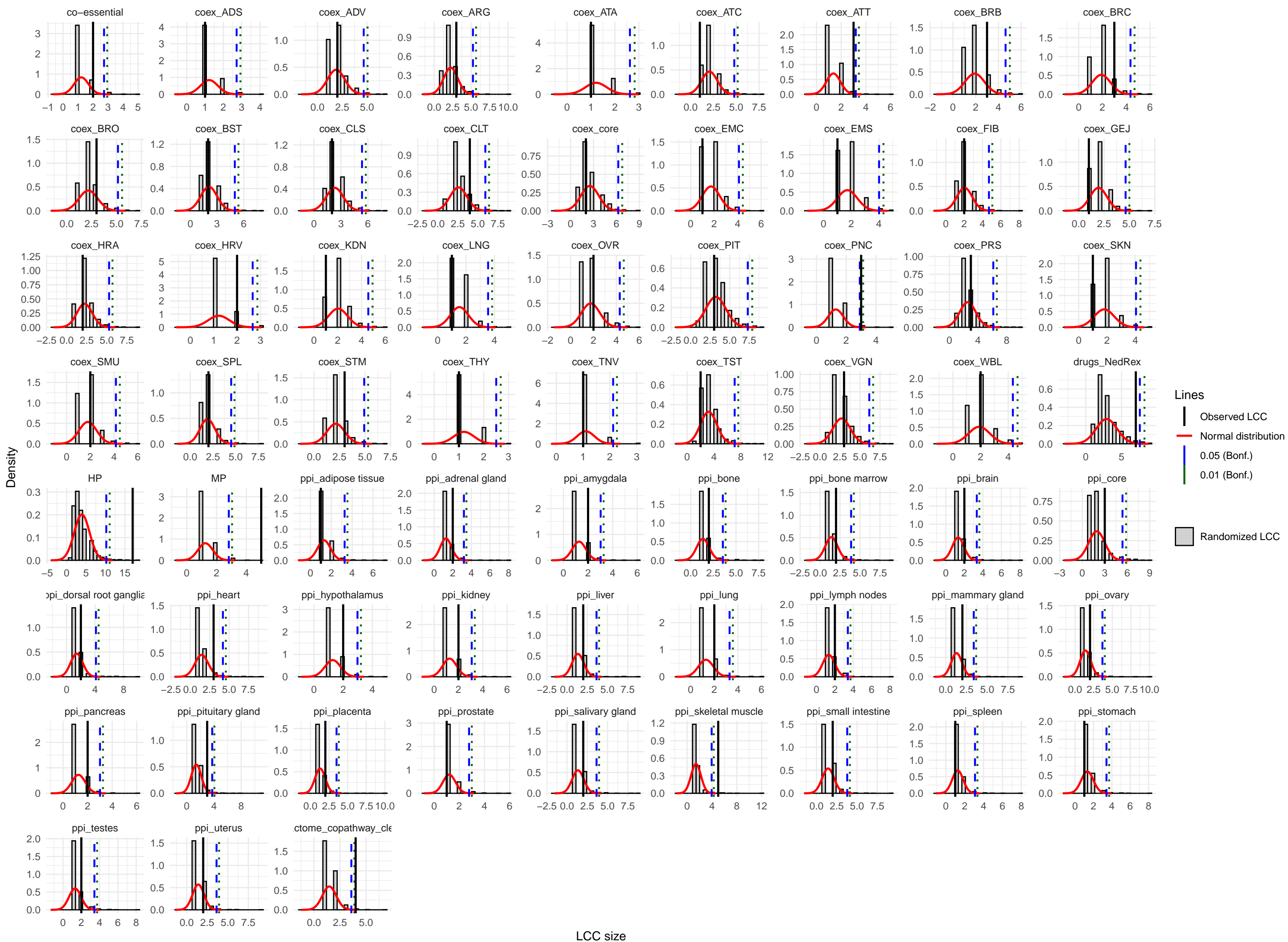
LCC distribution with normal curve and Bonferroni-corrected thresholds
