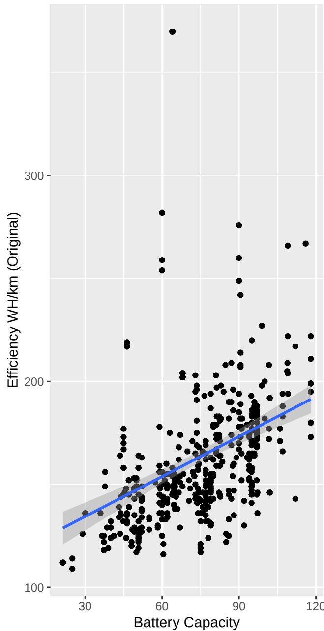
Battery Capacity and Efficiency WH/km regression
