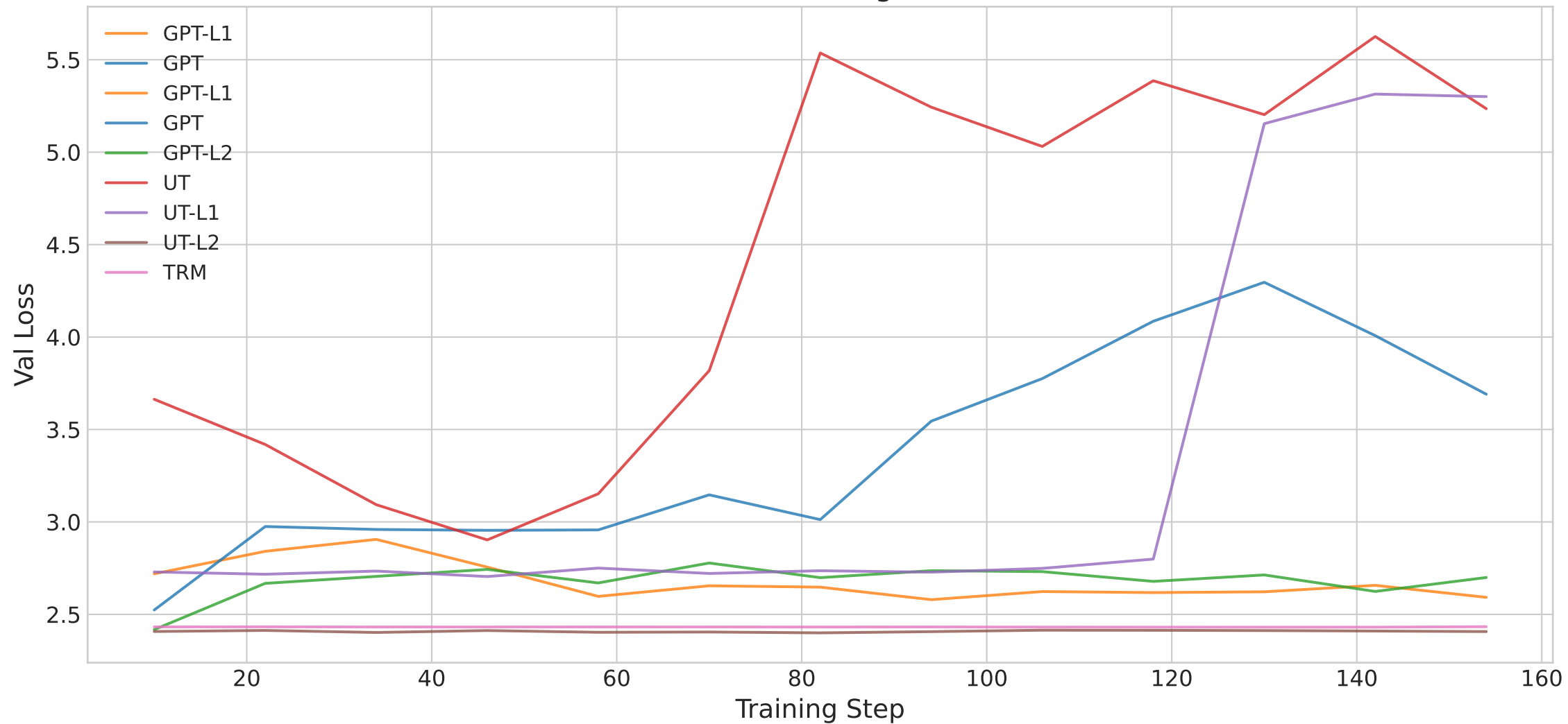
Addition: Training Curves
