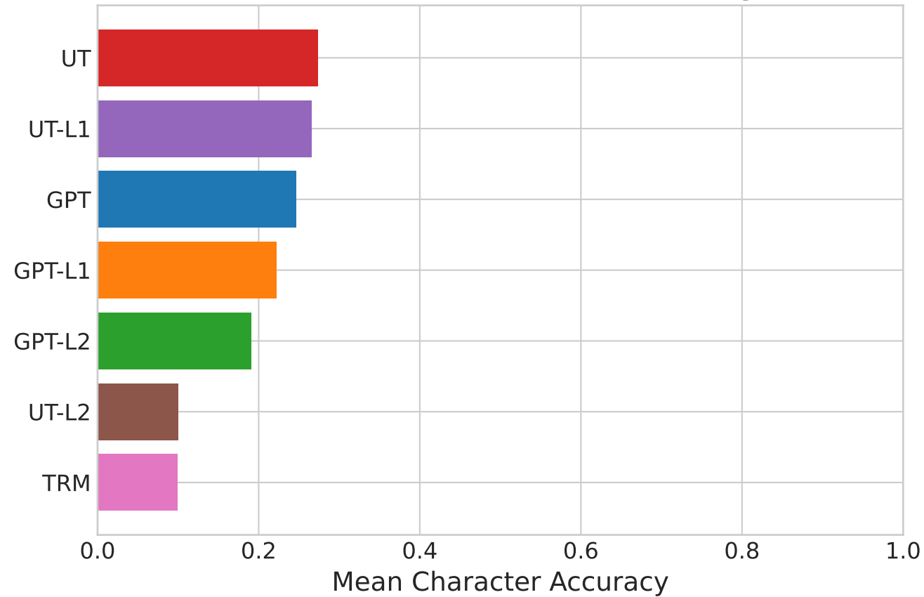
Overall Performance (All Tasks & Lengths)
