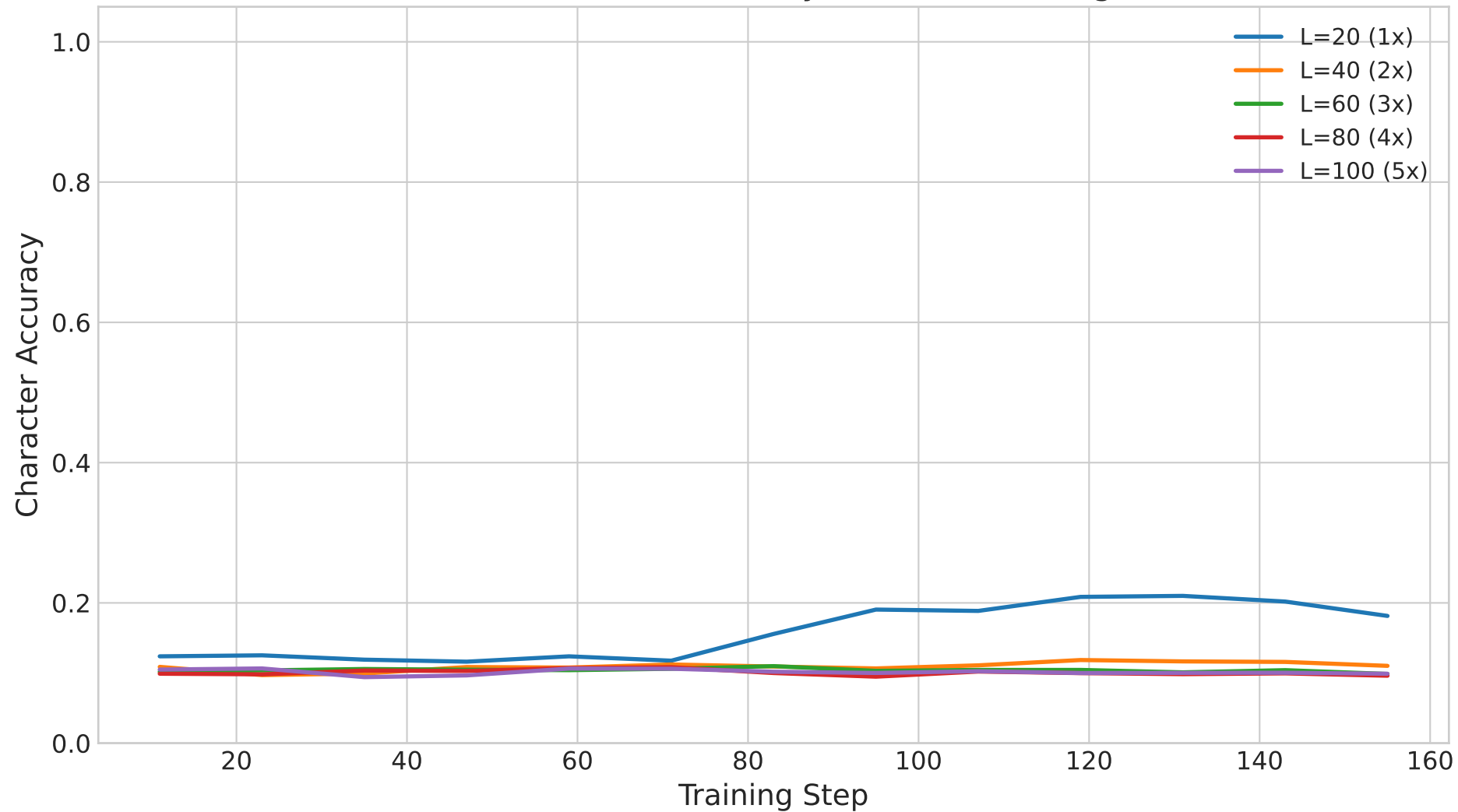
GPT on Addition: Accuracy at Different Lengths
