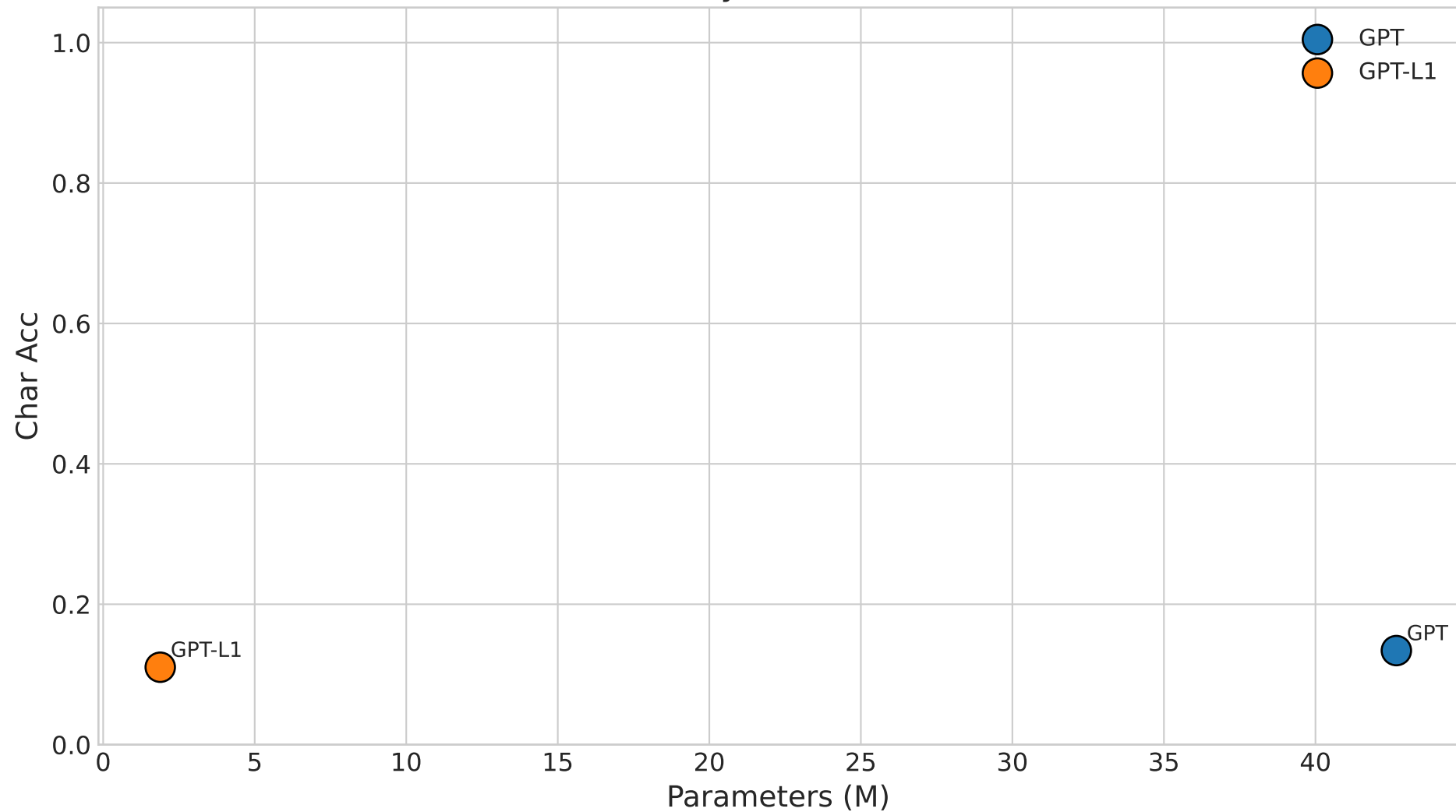
Reverse: Accuracy vs Model Size (L=100)
