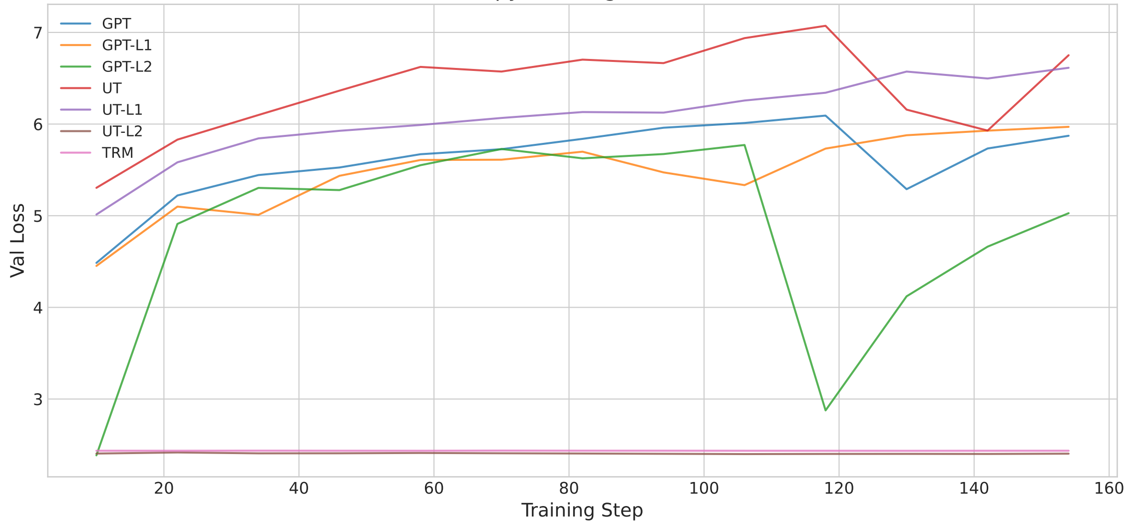
Copy: Training Curves
