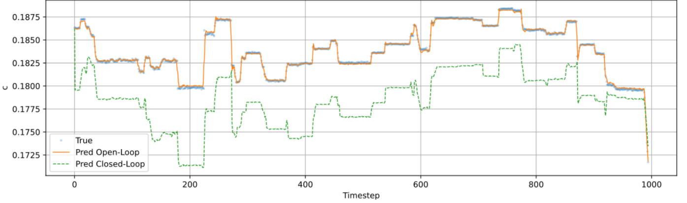
Fig. 5. Predicted concentration profile for the provided Beat-The-Felix trajectory in open- and closed-loop mode compared to the true values.
