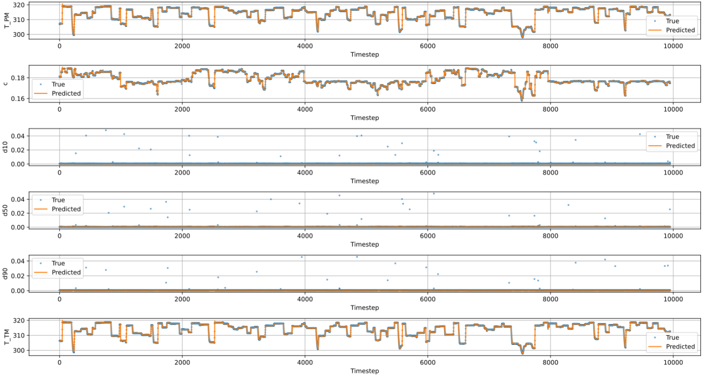
Fig. 3. Performance of the optimized NARX model for the test data set.
