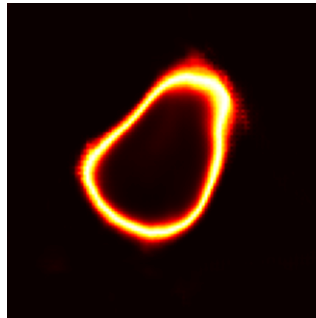
Entropy Map
