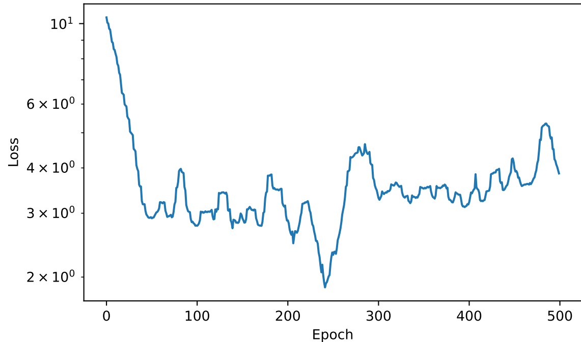
Training Loss
