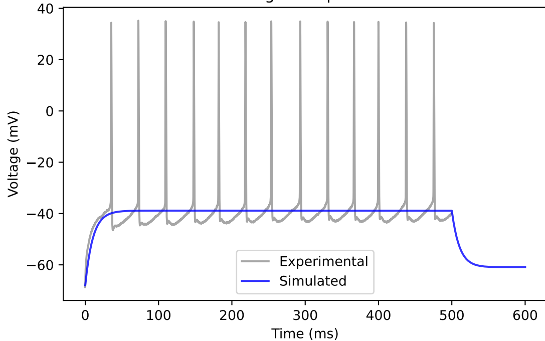
Voltage Comparison
