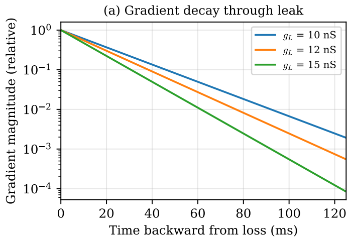
Figure 4.2: Vanishing Gradients Through Leak Dynamics
