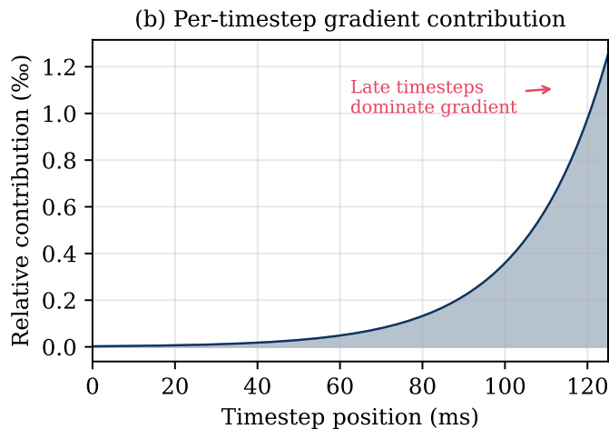
Figure 4.2: Vanishing Gradients Through Leak Dynamics
