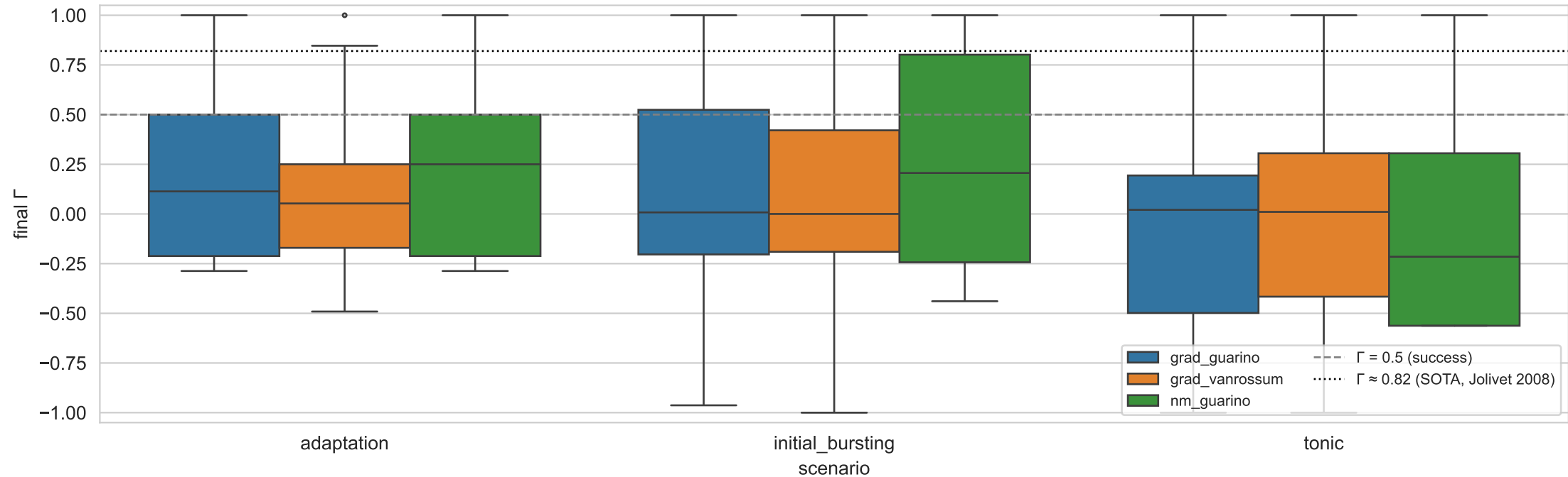
\Gamma distribution per (scenario, method) under warm-start protocol
