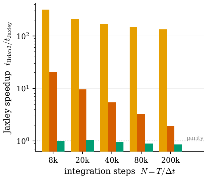
(b) Jaxley speedup vs each config
