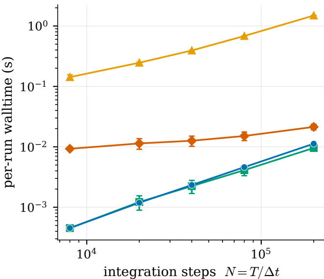
(a) absolute per-run walltime
