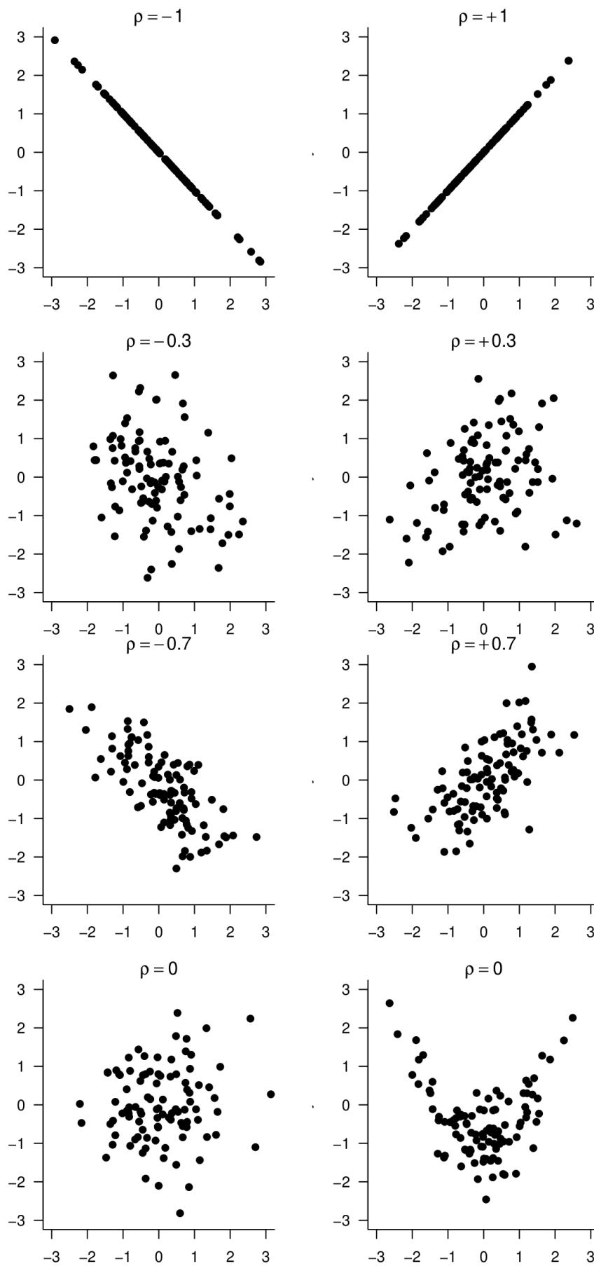
Figure 10.5: Samples from distributions with correlations \rho = 0 (2 of them), \rho = \pm 0.3 , \rho = \pm 0.7 and \rho = \pm 1 .
