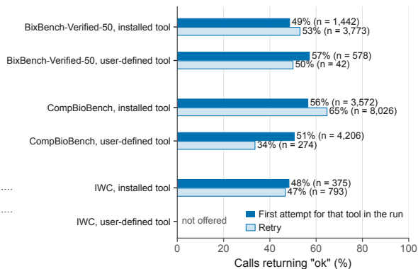
b Outcome of tool-tool calls: first attempts and retries
