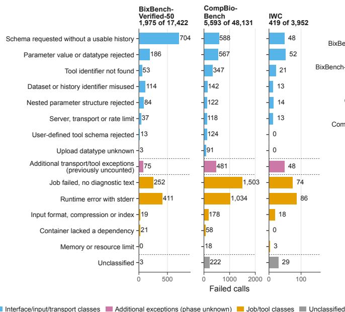
a Failed Galaxy-interface calls by class
