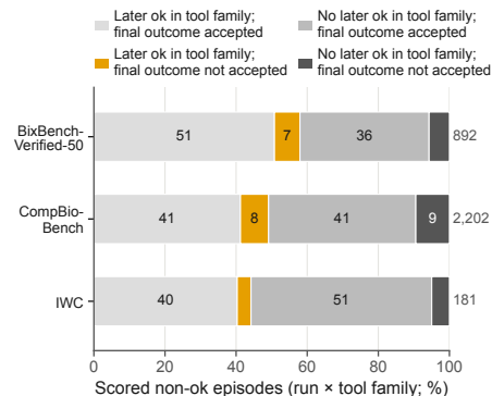
d After a non-ok tool call: later status and final evaluator outcome
