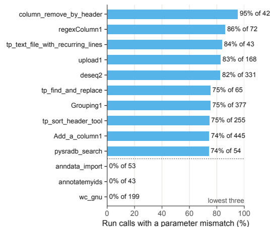
b Parameter-mismatch rate by tool (tools with ≥40 run calls)
