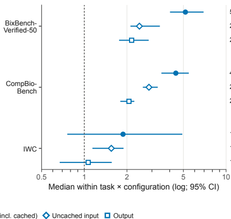
a Token use, Galaxy ÷ open-ended (complete cells)
