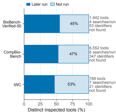
d Tools inspected and later run
