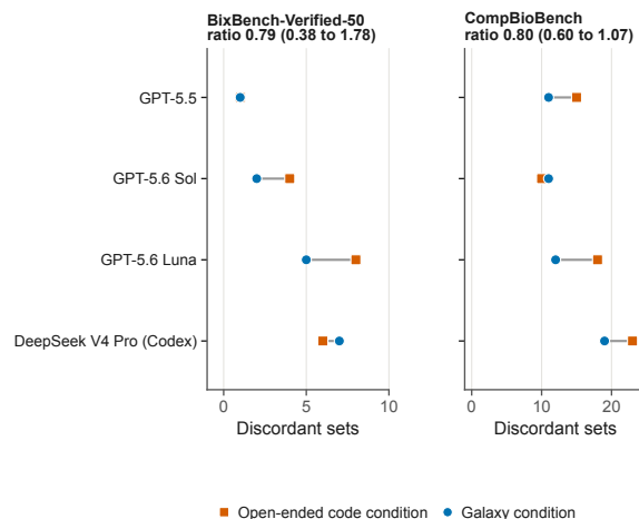
b Discordant replicate sets per model configuration
