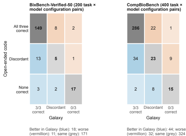
a Paired replicate-set outcomes, open-ended code to Galaxy
