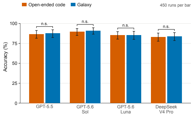
a Overall accuracy by model
