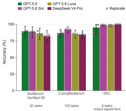
c Accuracy by benchmark and model in Galaxy
