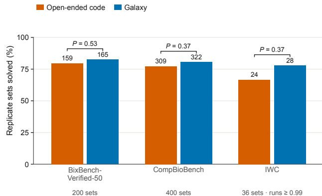
b Replicate sets with 3/3 correct
