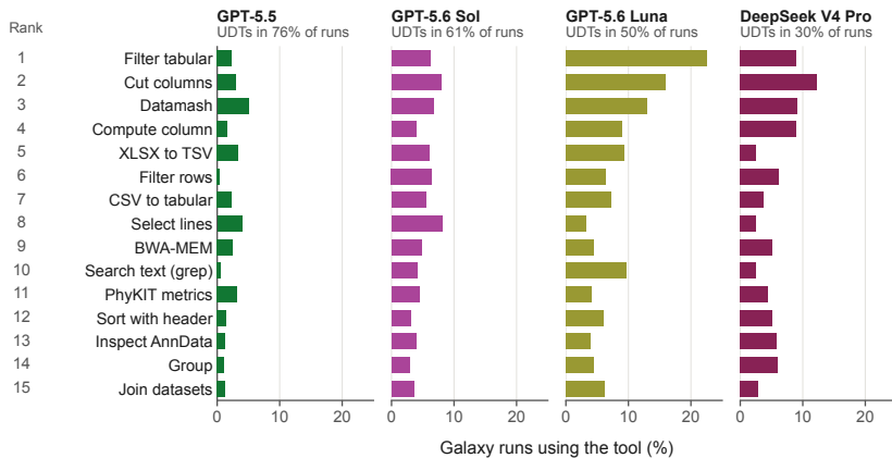
d 15 most used Galaxy tools
