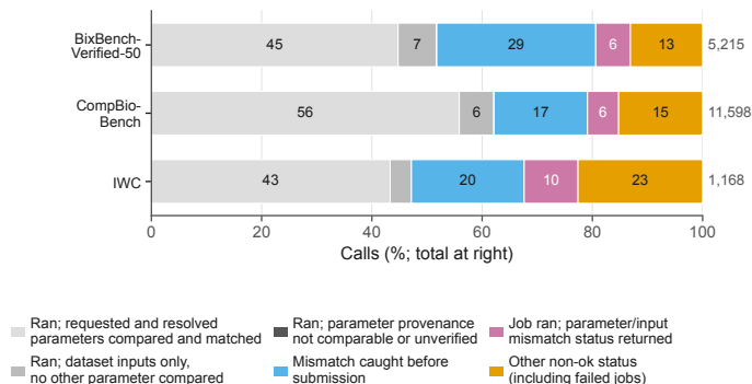
a Installed-tool run calls by parameter-check coverage and outcome
