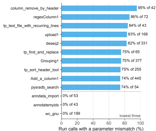
b Parameter-mismatch rate by tool (tools with \geq 40 run calls)
