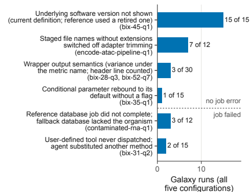
d Galaxy-specific mechanisms behind scored-incorrect runs
