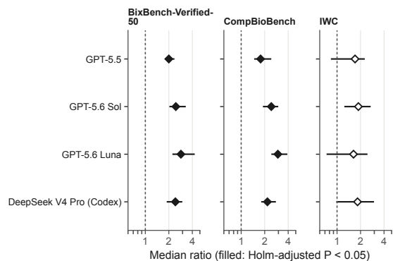
c Actions per run, Galaxy ÷ open-ended code
