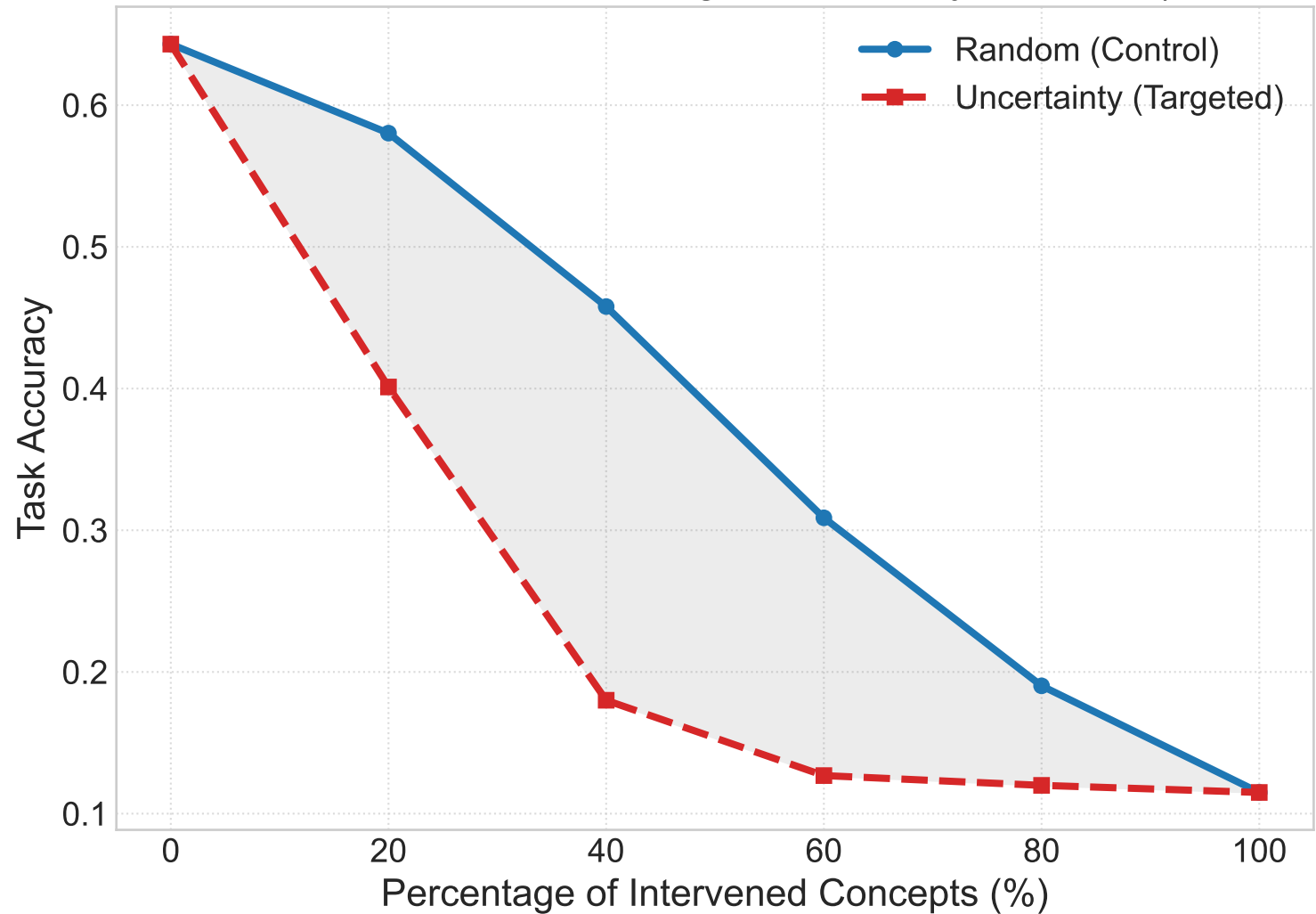
Causal Intervention: The Leakage/Uncertainty Paradox ( \lambda = 0.5 )
