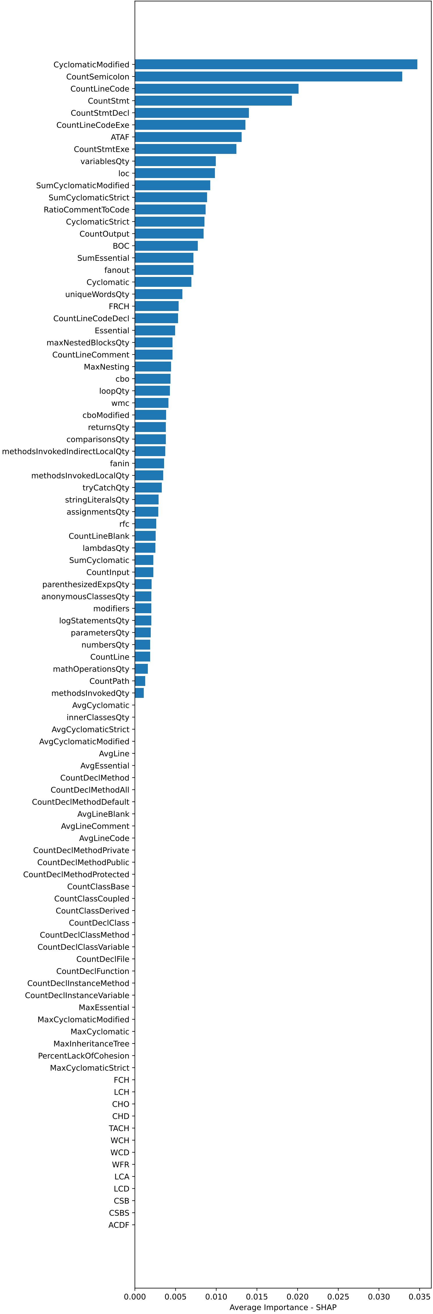
Feature Ranking - SHAP
