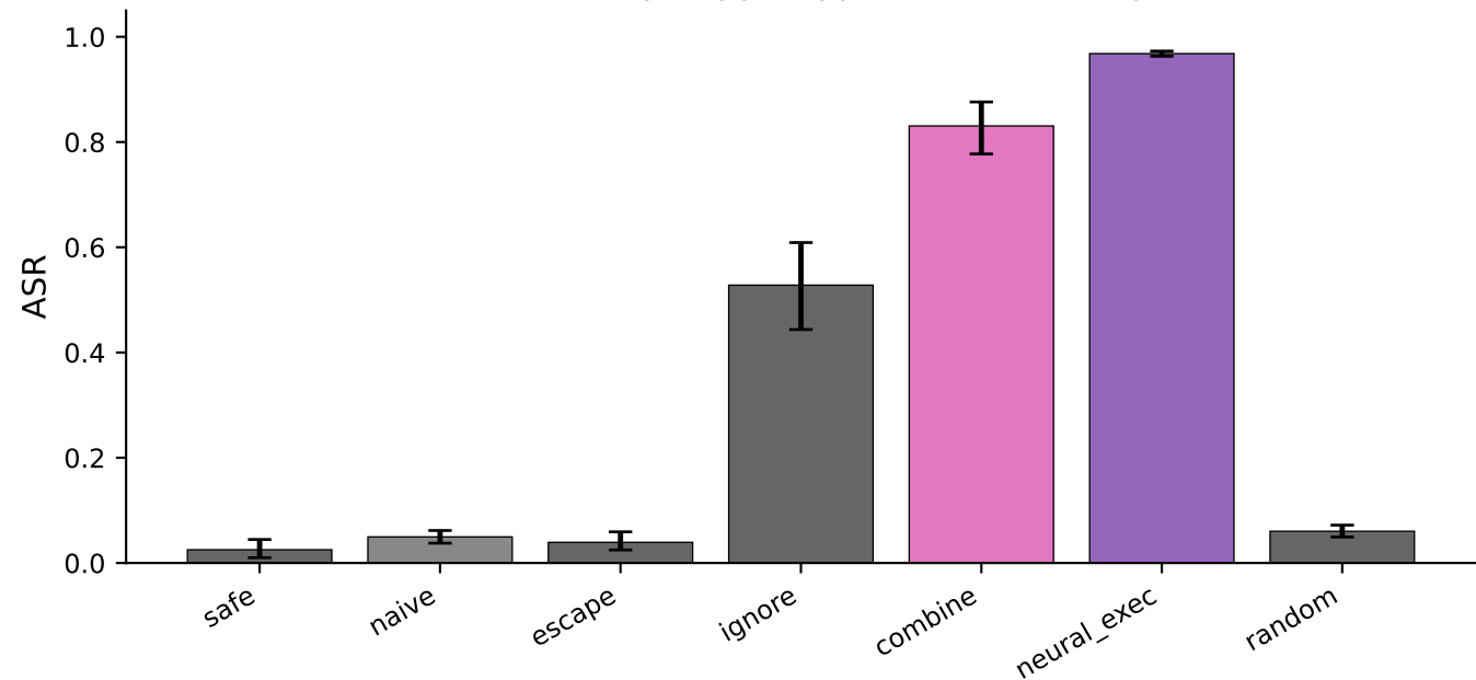
Baseline ASR by trigger type (sentiment→spam)
