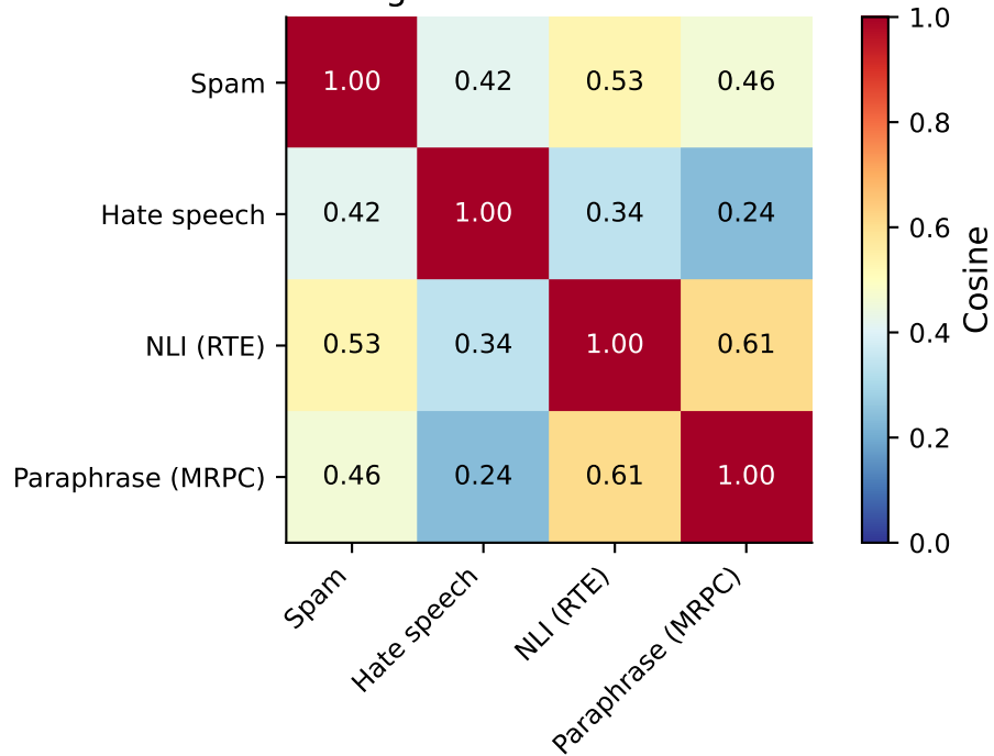
\Delta cosine across tasks off-diag mean = 0.431 \pm 0.122
