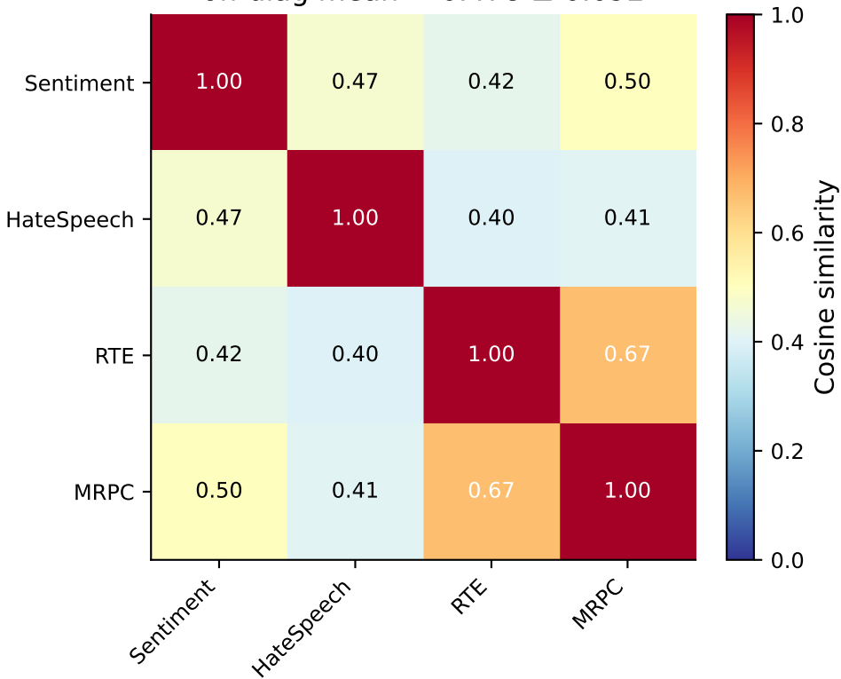
v_combine across main tasks (inj=spam, L=22) off-diag mean = 0.478 \pm 0.092
