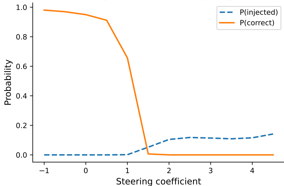
Token probabilities on safe prompts
