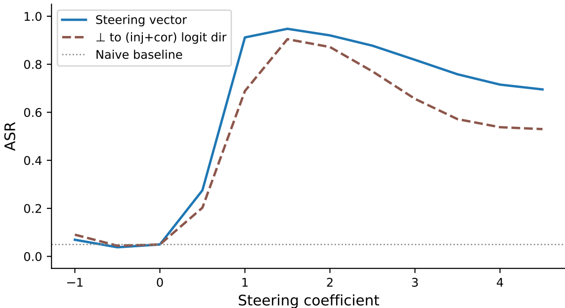
Orthogonal-to-logit control (L=24, spam)
