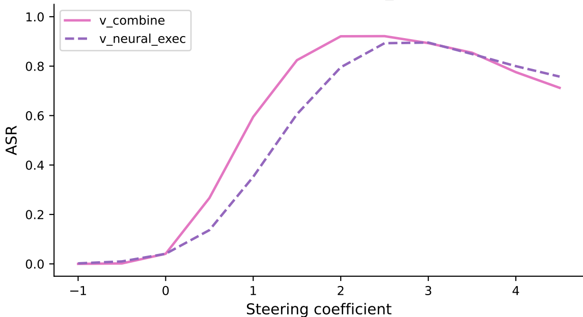
Steering naive prompts: combine vs neural_exec vector (L=21, spam)
