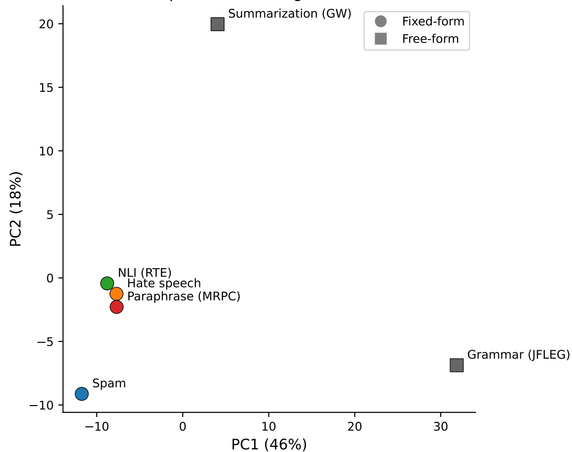
PCA of per-task steering vectors (L=21)
