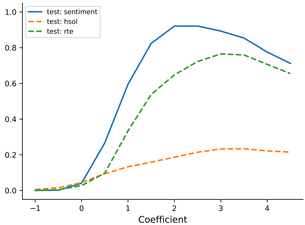
Train: sentiment
