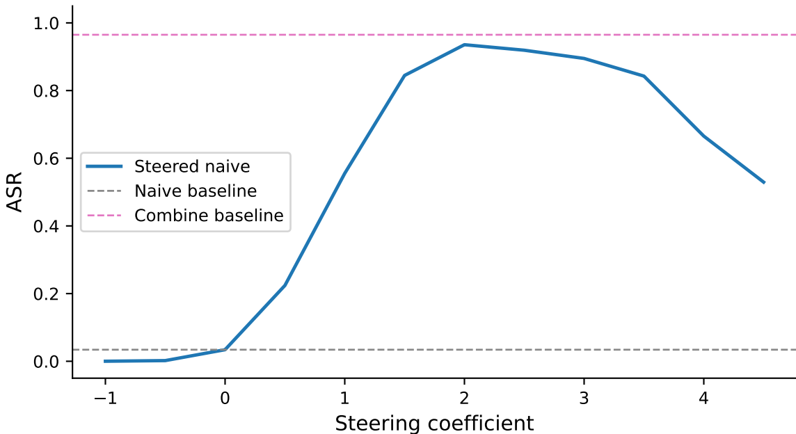
Sufficiency: steering naive→combine (L=21, spam)
