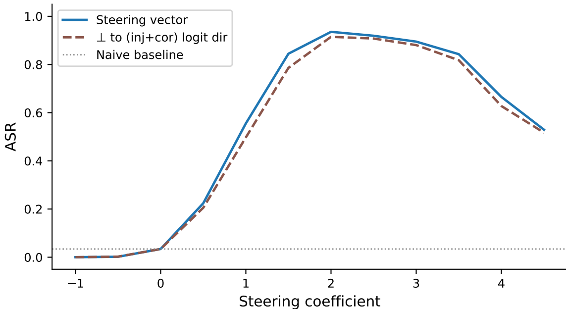
Orthogonal-to-logit control (L=21, spam)
