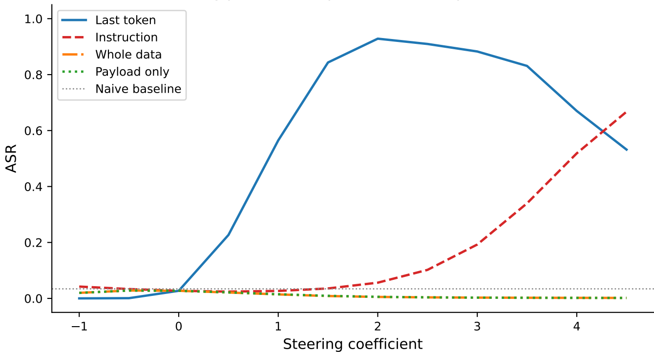
Steering position comparison (L=21, spam, n=50)
