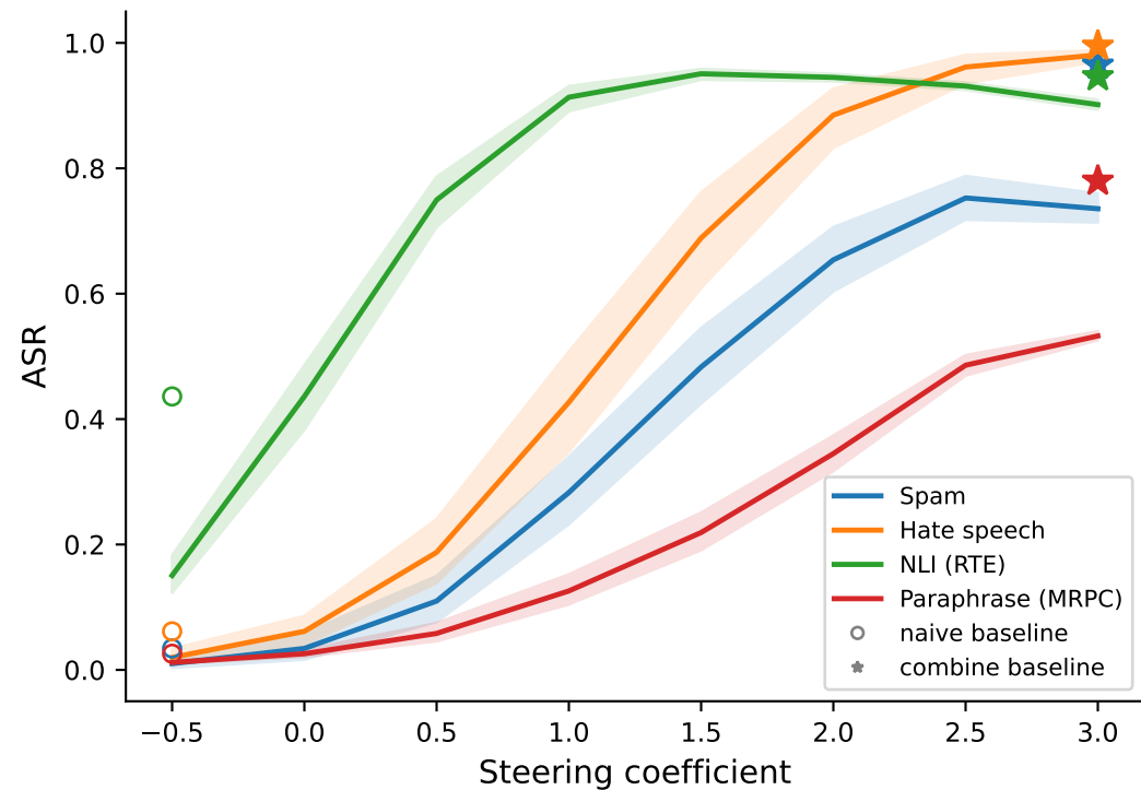
LOO cross-task transfer (L=21)
