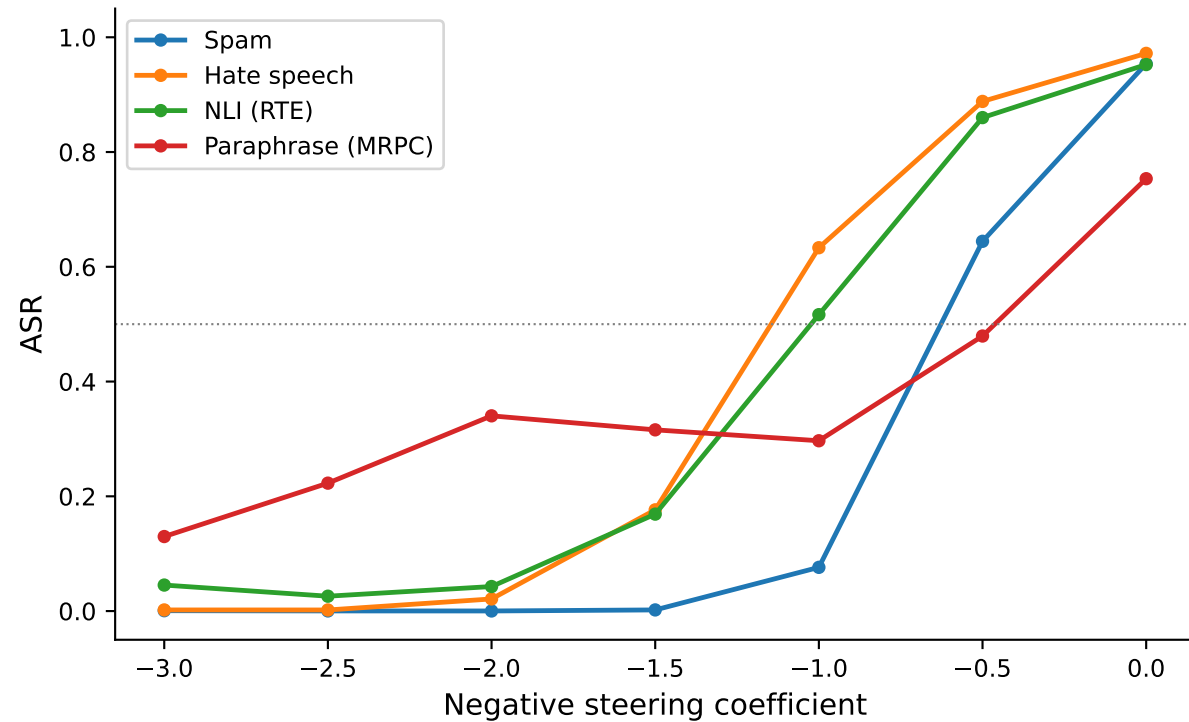
Ablation with Spam vector
