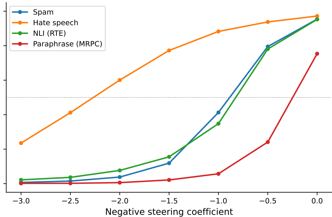
Ablation with Paraphrase (MRPC) vector
