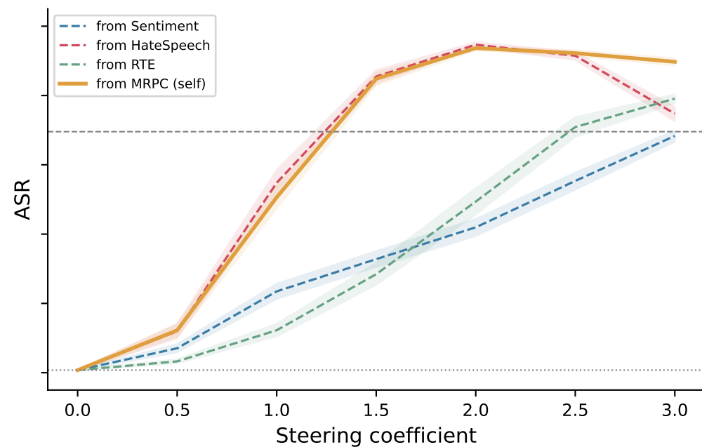
Test: MRPC
