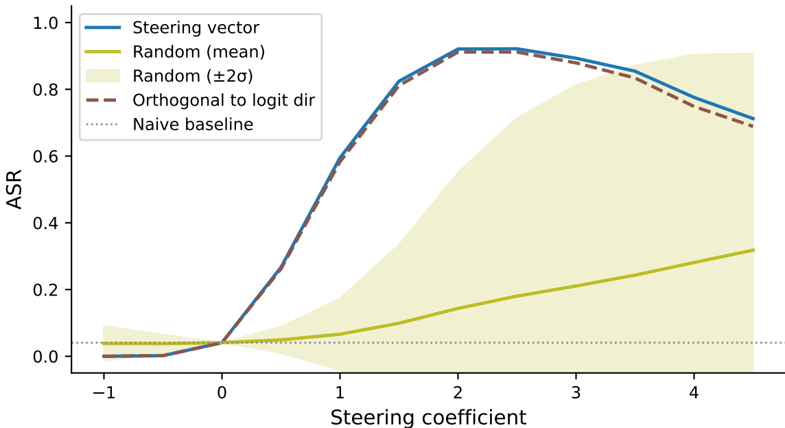
Controls (L=21, spam)
