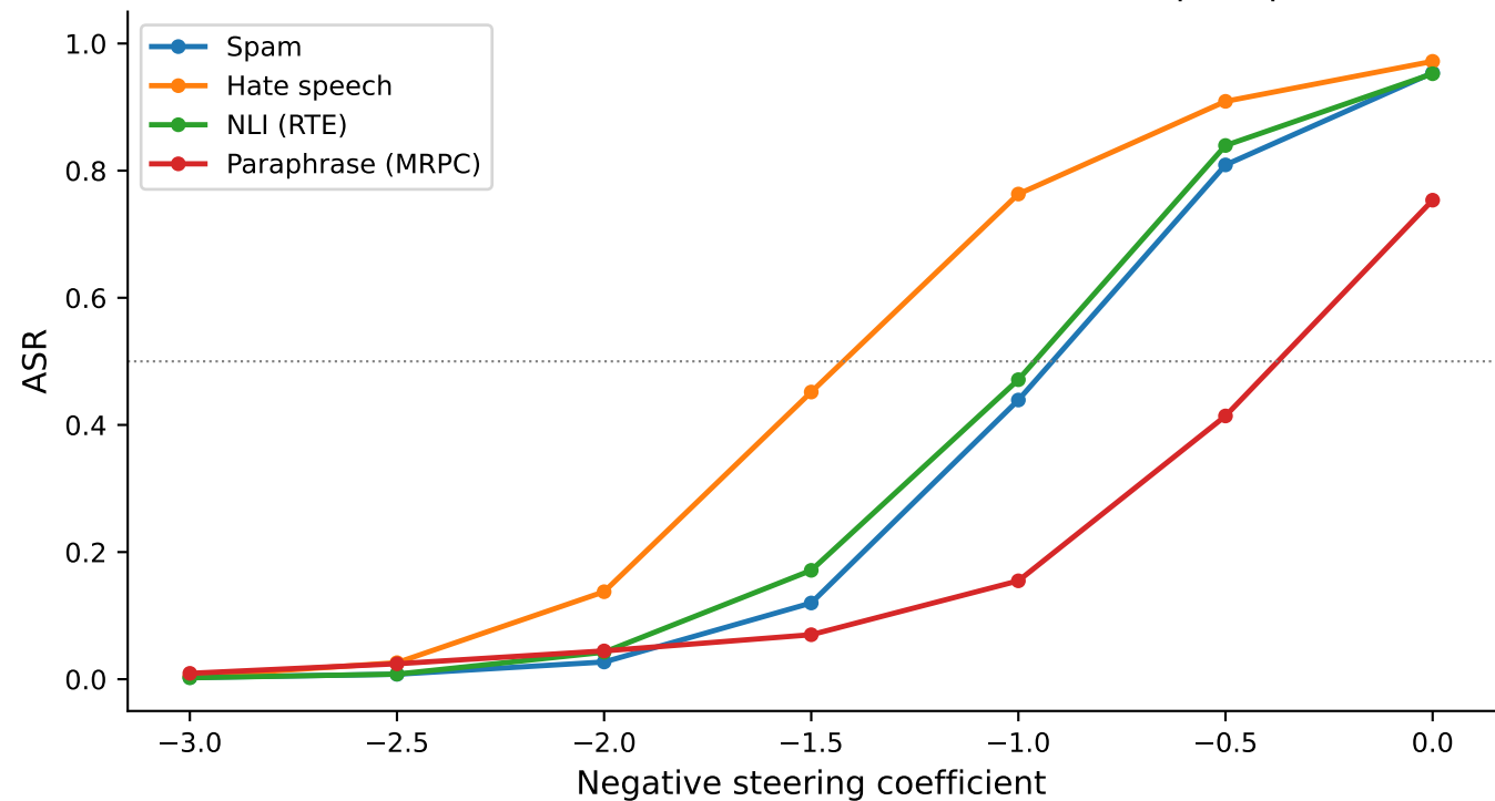
LOO ablation (shared vector on held-out combine prompts)
