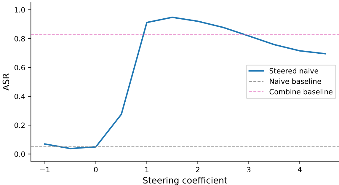
Sufficiency: steering naive→combine (L=24, spam)
