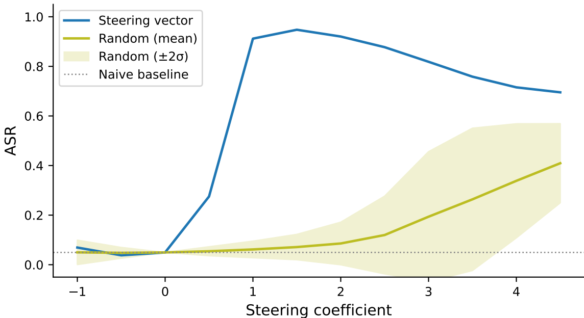
Random-vector control (L=24, spam)
