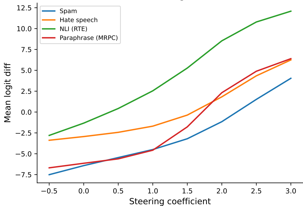
LOO cross-task logit difference
