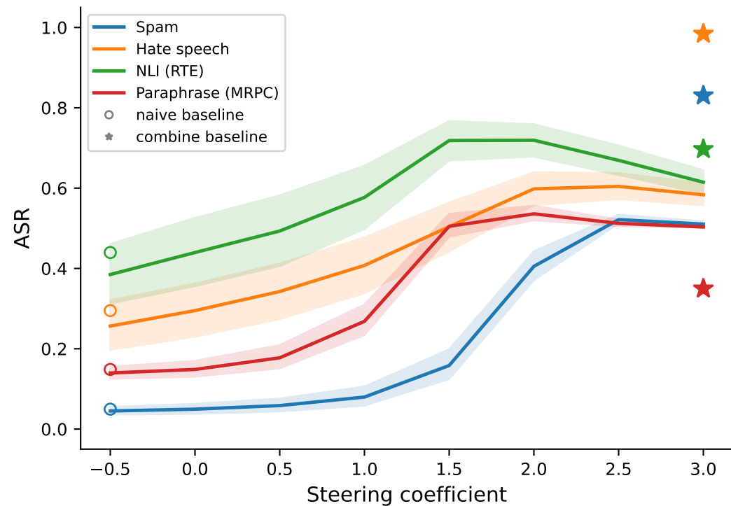
LOO cross-task transfer (L=24)
