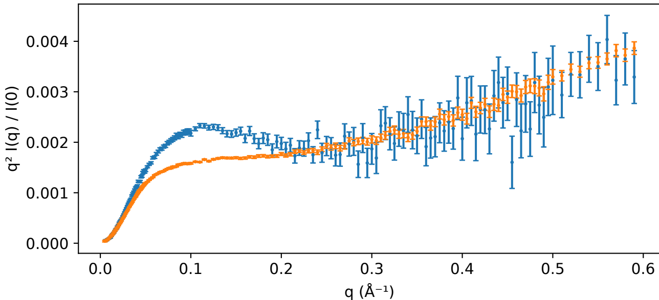
High- q Kratky — \pm 1\sigma at fixed normalization
