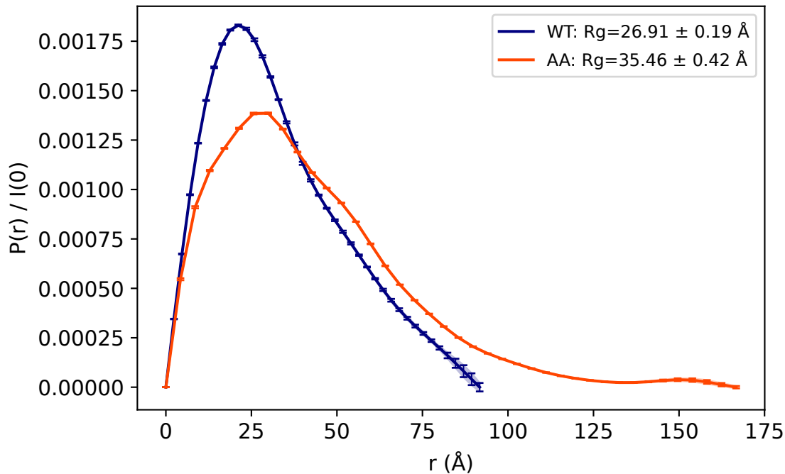
Pair-distance distribution — BIFT
