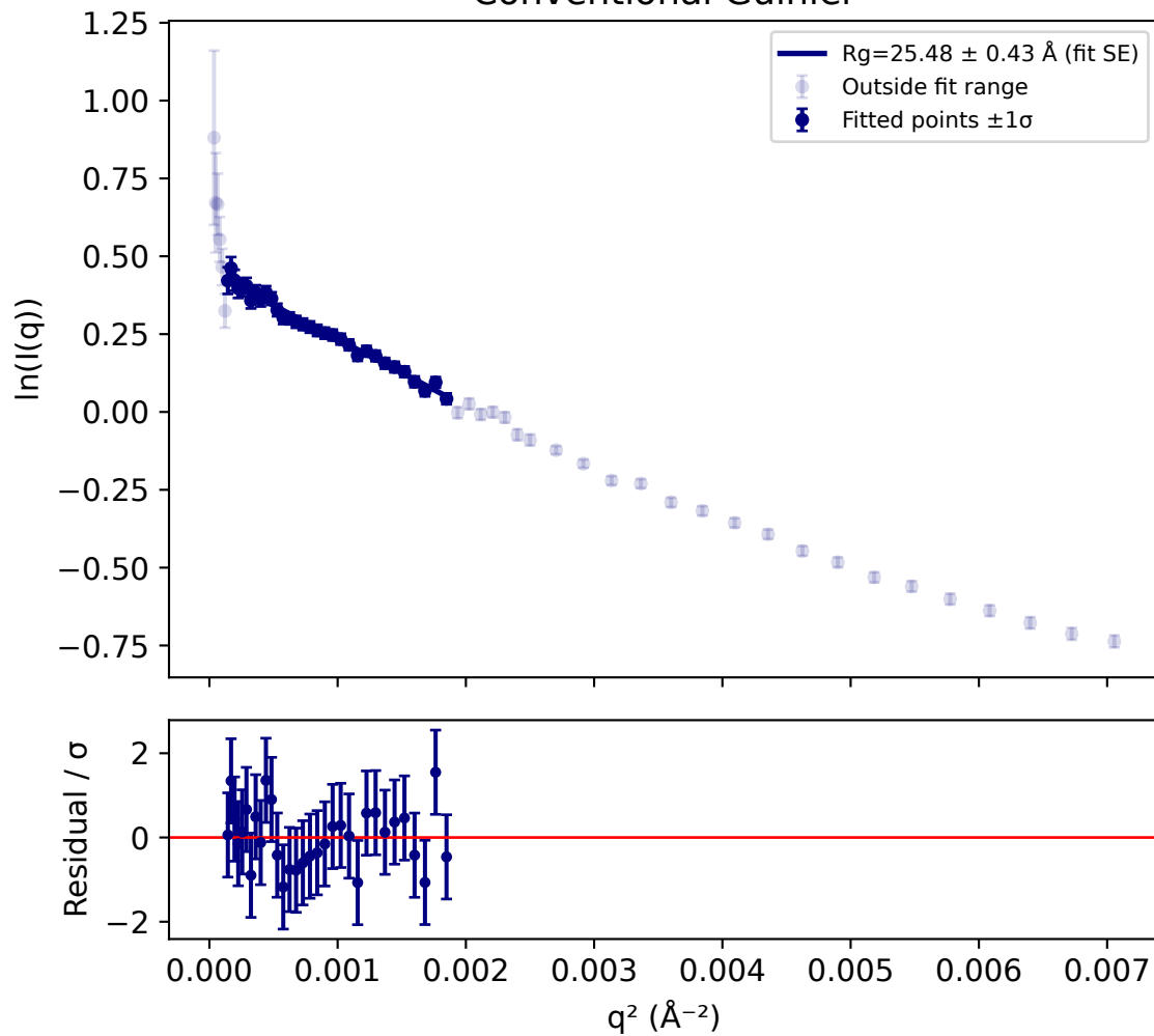
Conventional Guinier
