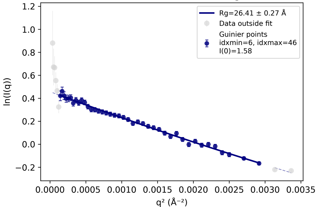
Extended Guinier Fit for WT Average Profile
