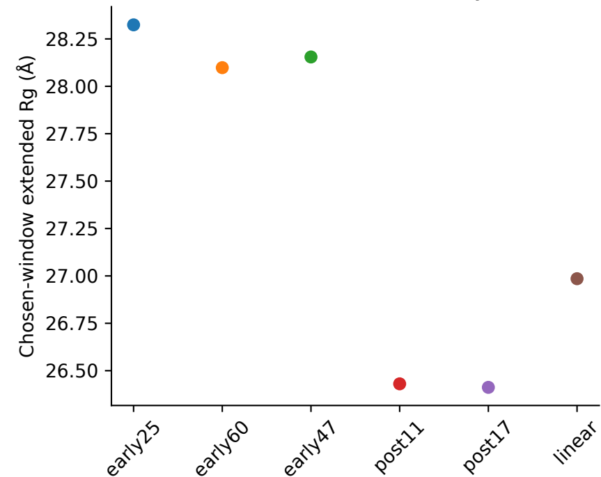
Buffer-model sensitivity
