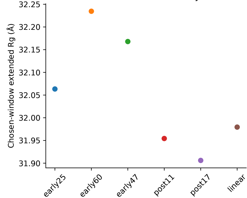
Buffer-model sensitivity
