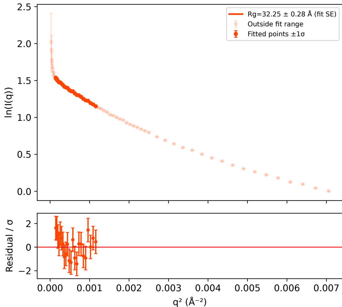
Conventional Guinier
